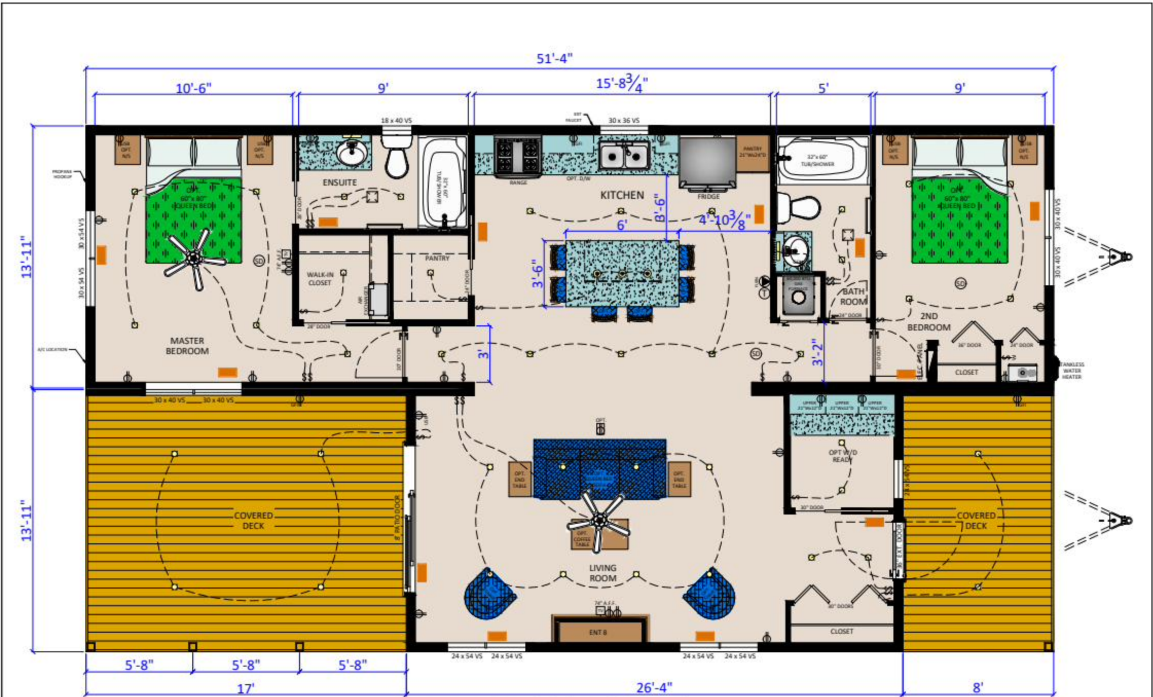
PARTRIDGE - 26 (P5128 2 BR) (1080.9 SQ.FT.) STANDARD CSA-Z240MH
