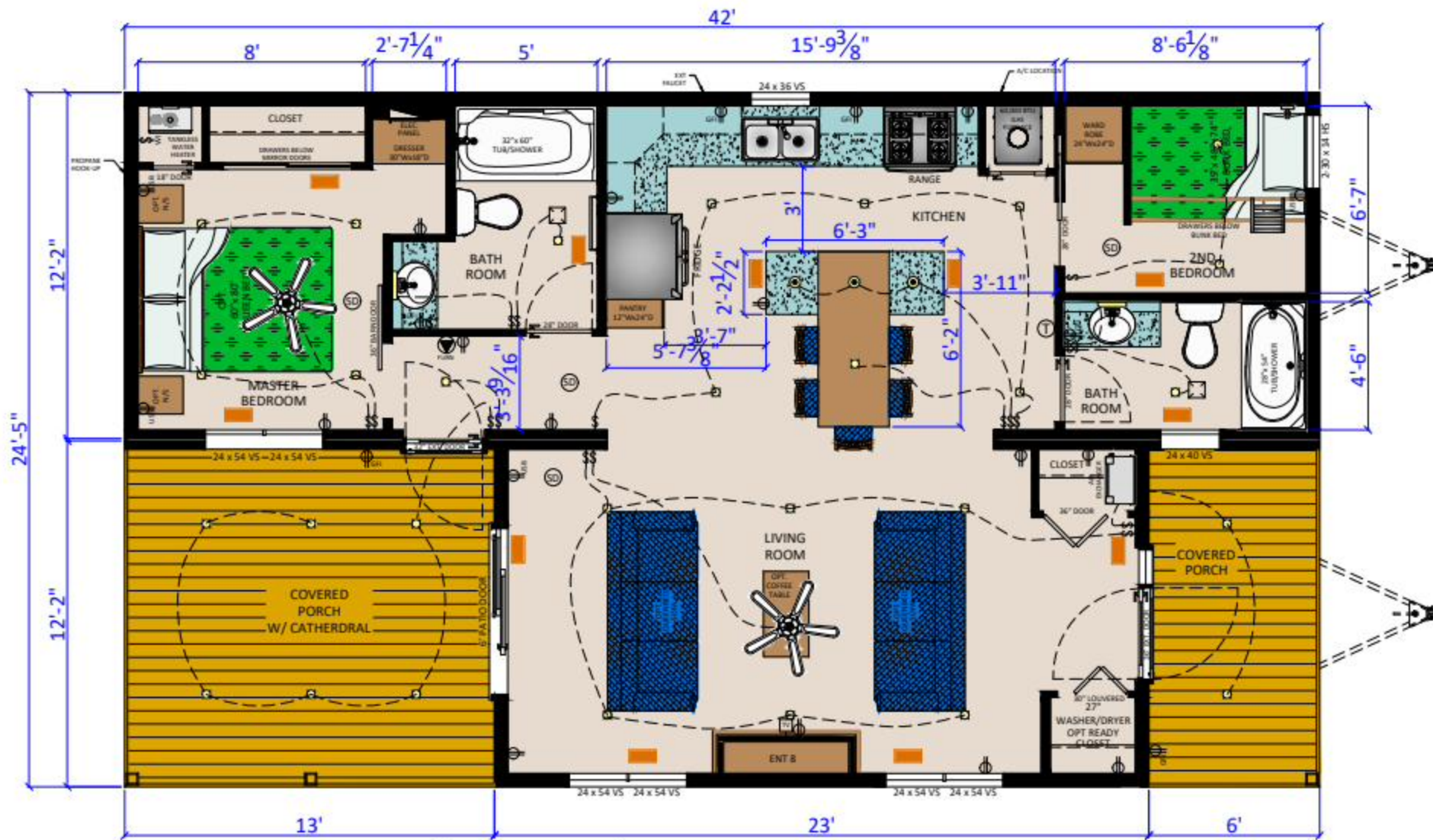
PENETANGORE - 26 (P4224 2 BR) (790.7 SQ.FT.) STANDARD CSA-Z240MH
