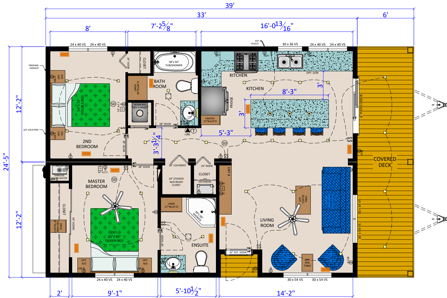
PENTICTON - 26 (P3824 2BR) (912 SQ.FT.) STANDARD CSA-Z240MH
