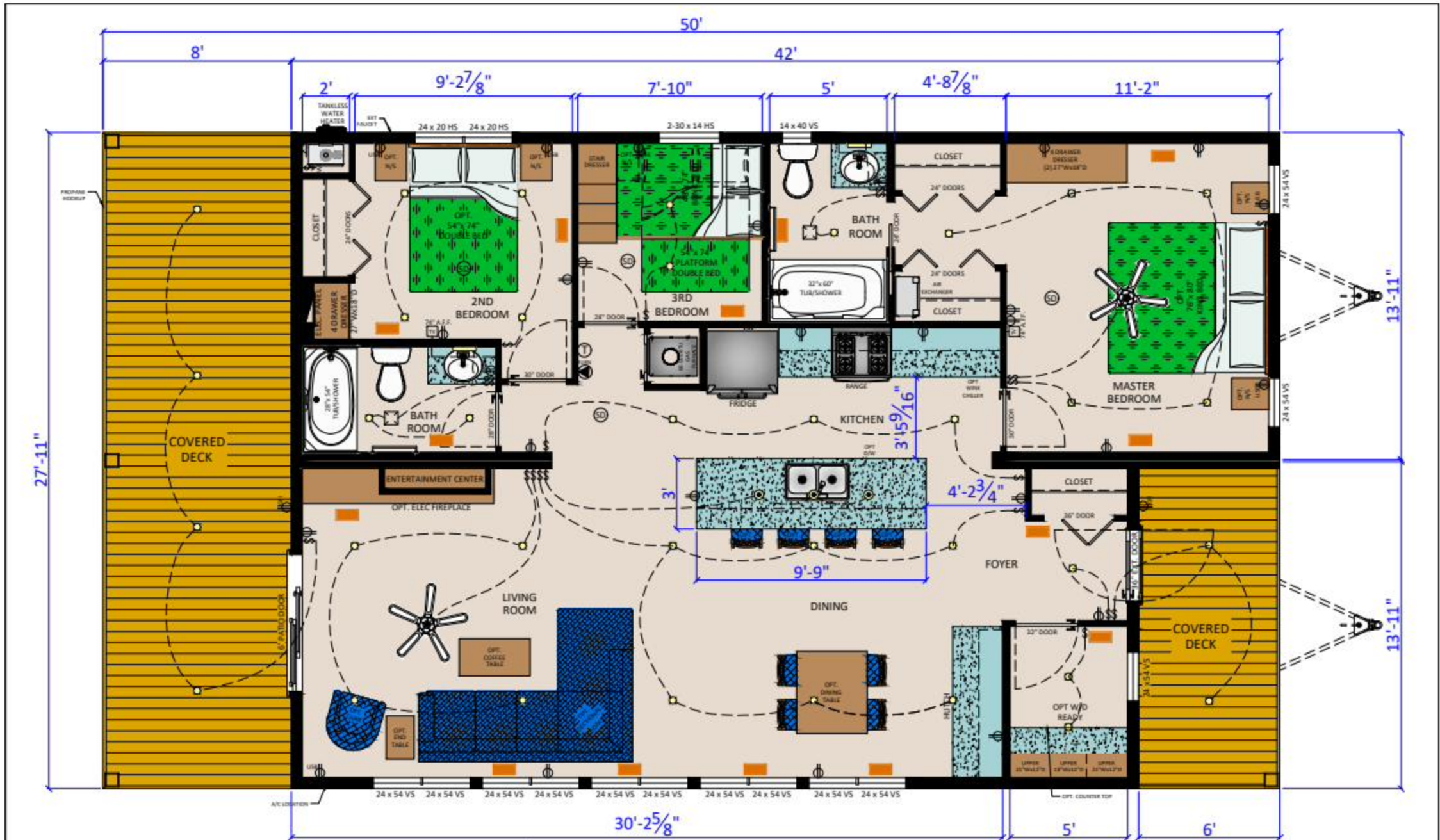
PICKWORTH - 26 (5028 3 BR) (1086.3 SQ.FT.) STANDARD CSA-Z240MH
