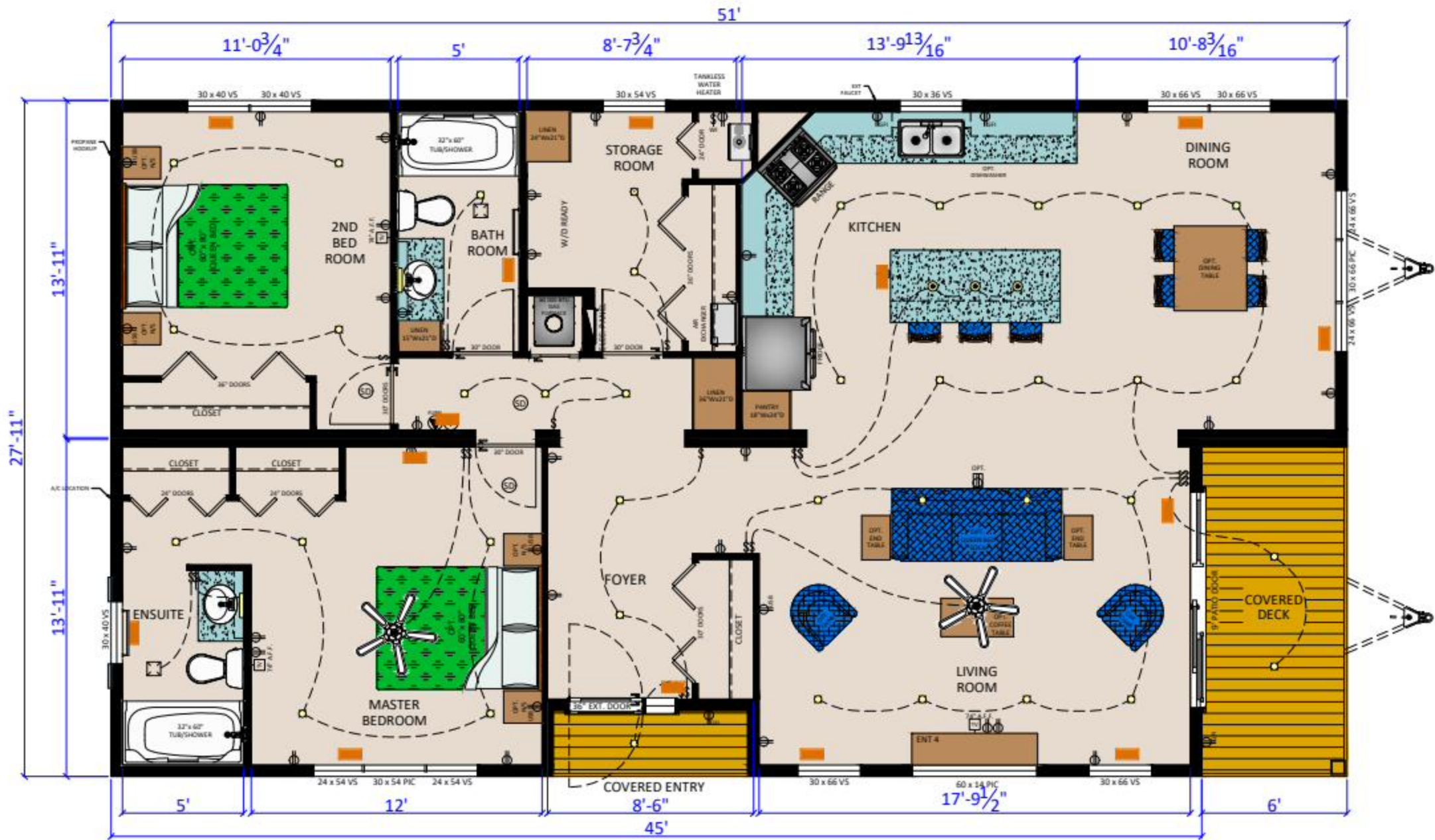
PROSPECT - 26 (P5128 2BR) (1315.3 SQ.FT.) STANDARD CSA-Z240MH
